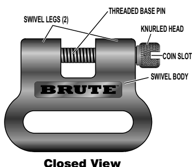
The BRUTE E-Z Detachable Sling Swivels (See pictorials to identify the BRUTE Sling Swivel Parts)
